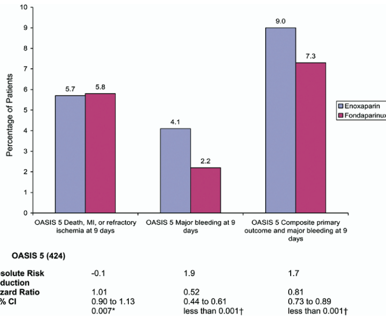
Figure 15. OASIS 5 Cumulative Risks of Death, MI, or Refractory Ischemia
