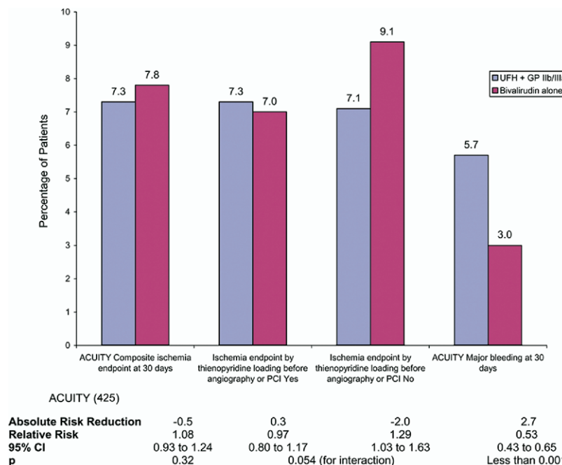
Figure 14. ACUITY Composite Ischemia and Bleeding Outcomes
